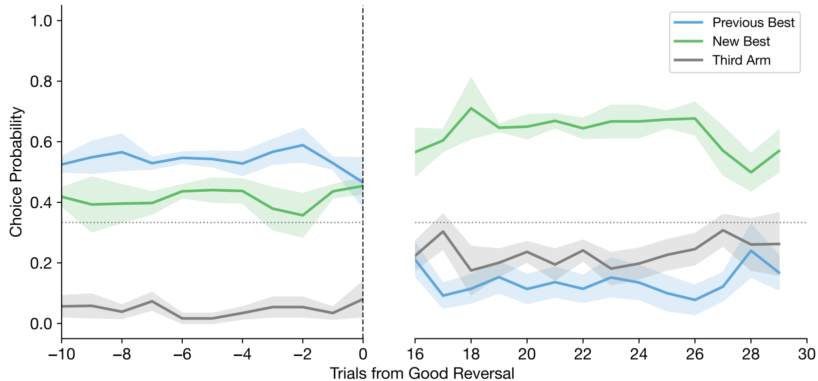
Good Reversal-Aligned Choices (mean \pm se across subjects | n=4 subjects, n=45 reversals) (Skipping first 15 trials post-reversal)
